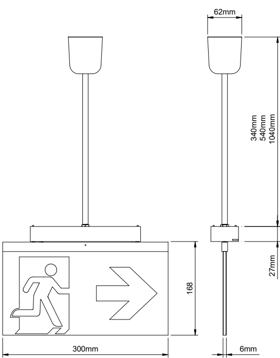
Pole suspension mounting
