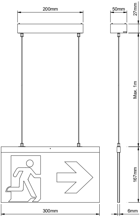
Wire suspension mounting
