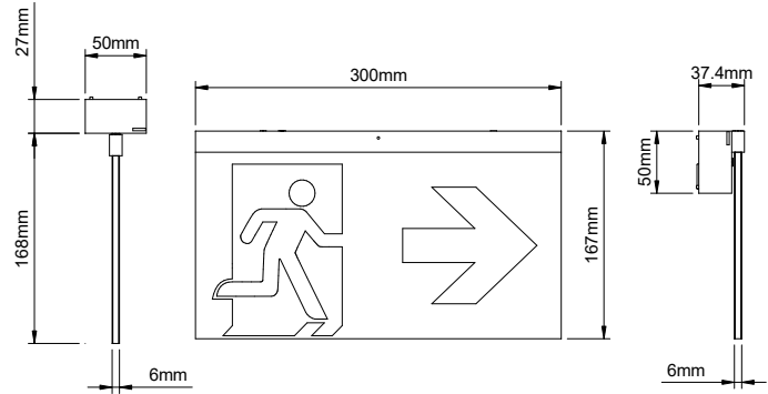
Wall-surface mounting
