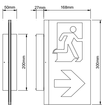
Vertical wall mounting
