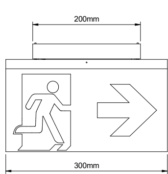
Ceiling-surface mounting
