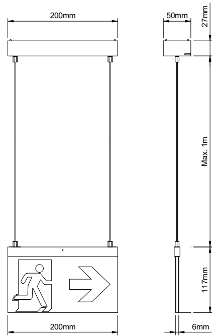
Wire suspension mounting
